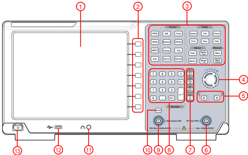
Figure 4-1 Front panel
